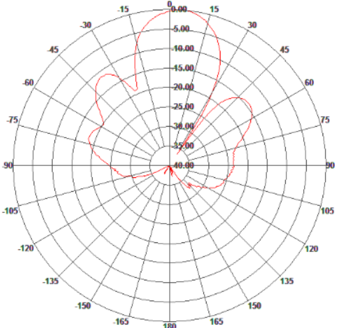
Elevation Pattern
