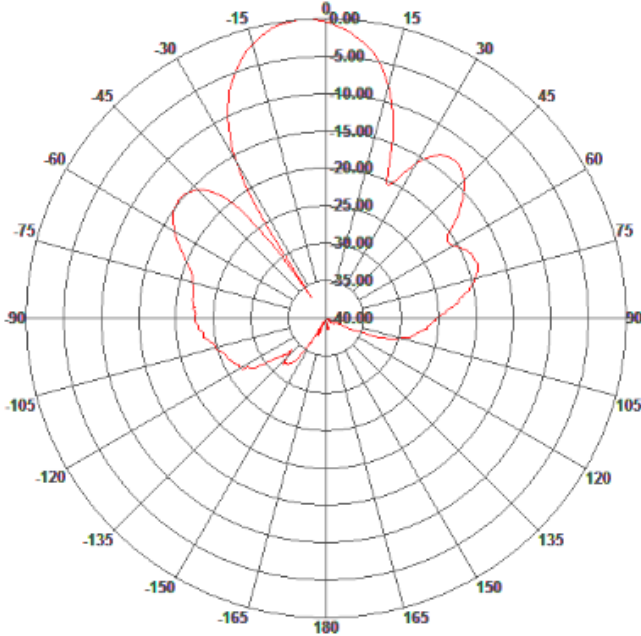
Azimuth Pattern
