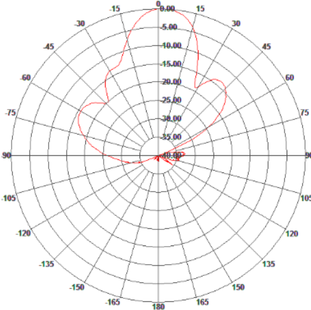
Azimuth Pattern
