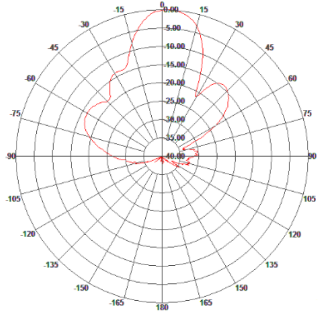
Elevation Pattern
